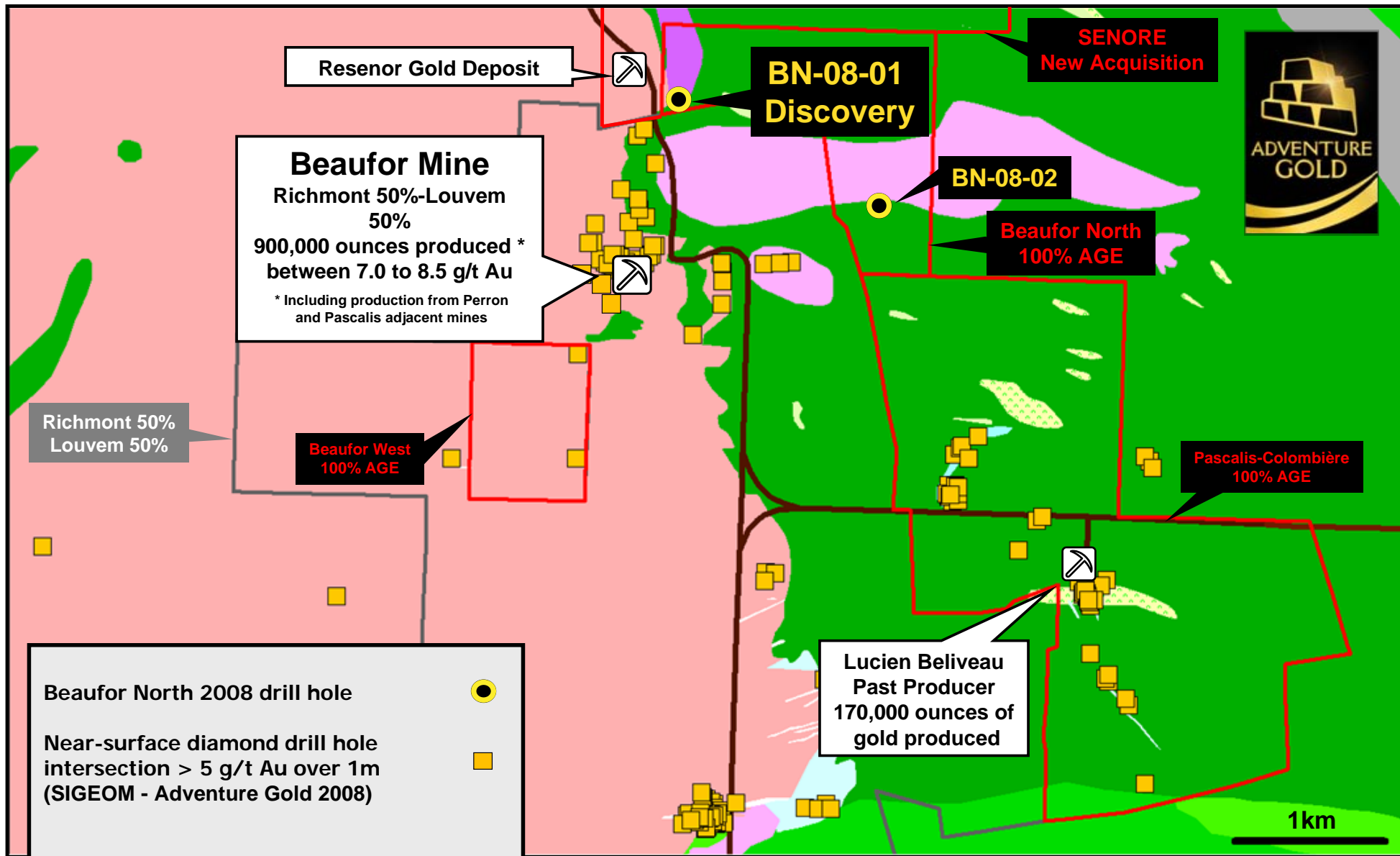
Figure 1: Adventure Gold 2008 drill hole location at Beaufor North – Gold distribution near-surface
