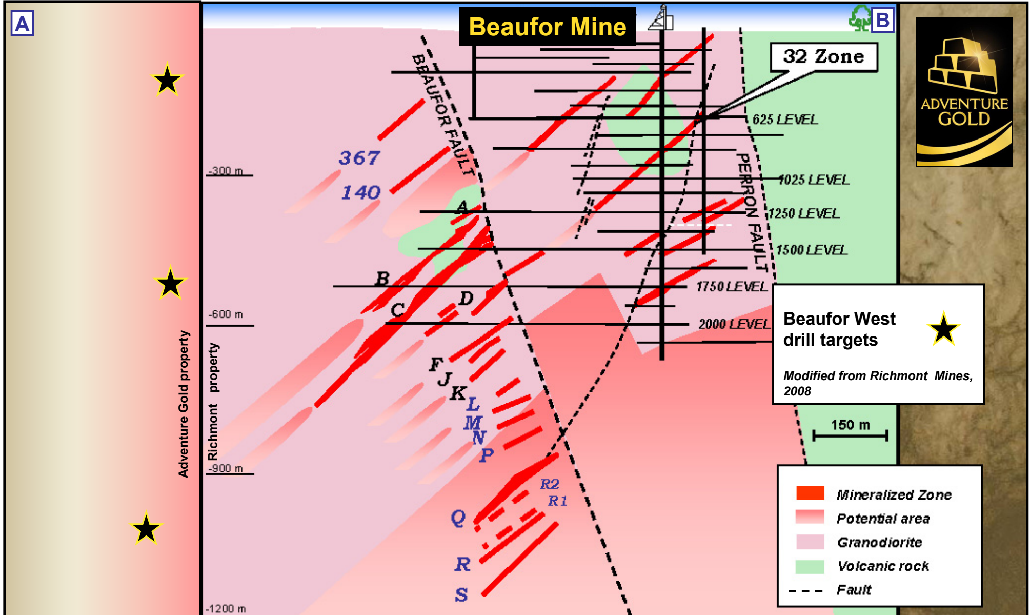
Figure 2: Adventure Gold 2008 drill targets at Beaufor West – Vertical section showing the gold-bearing veins at the Beaufor Mine
