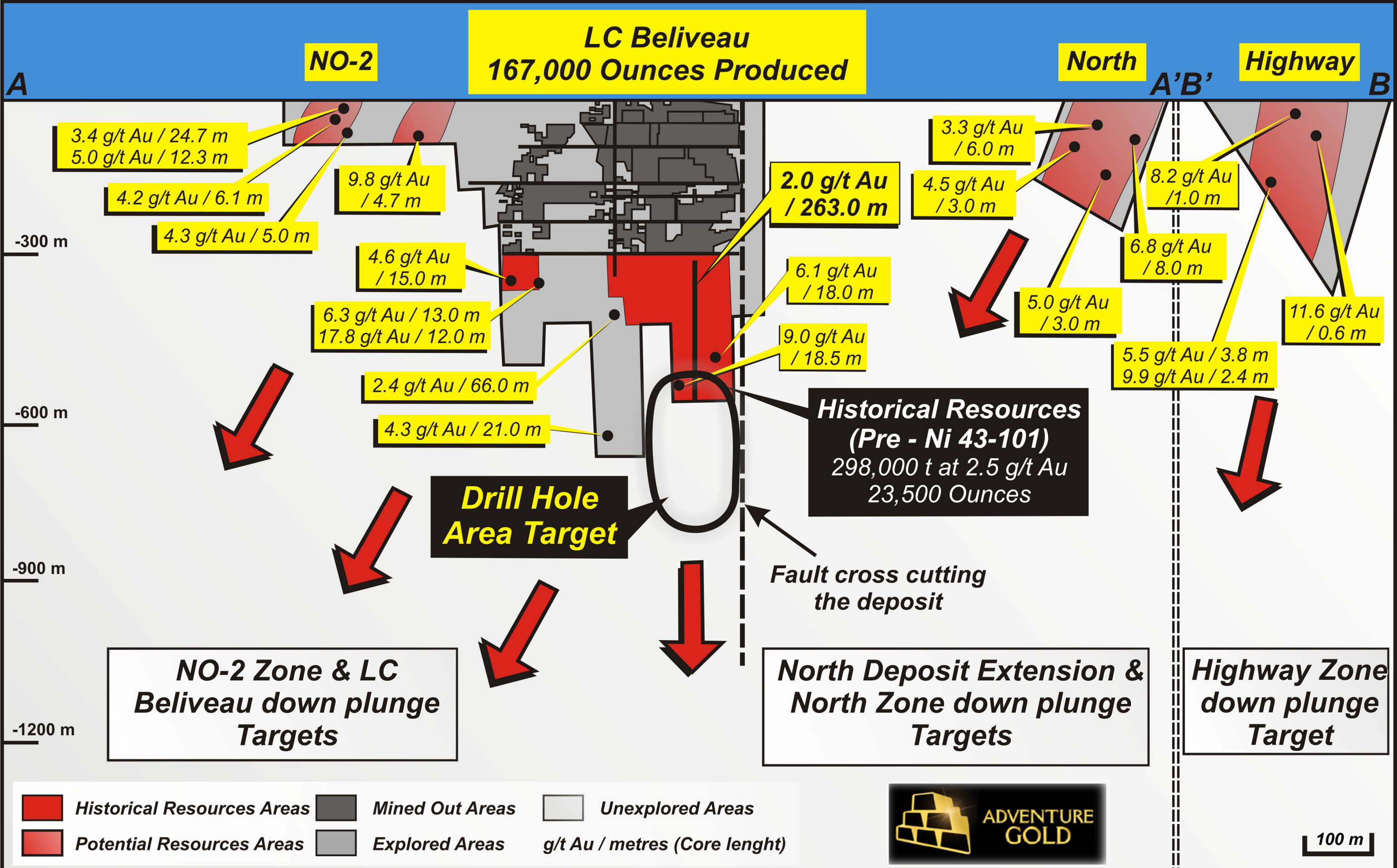
Figure 1: Schematic NS Vertical Longitudinal Section – Drilling Target Area Phase 1
