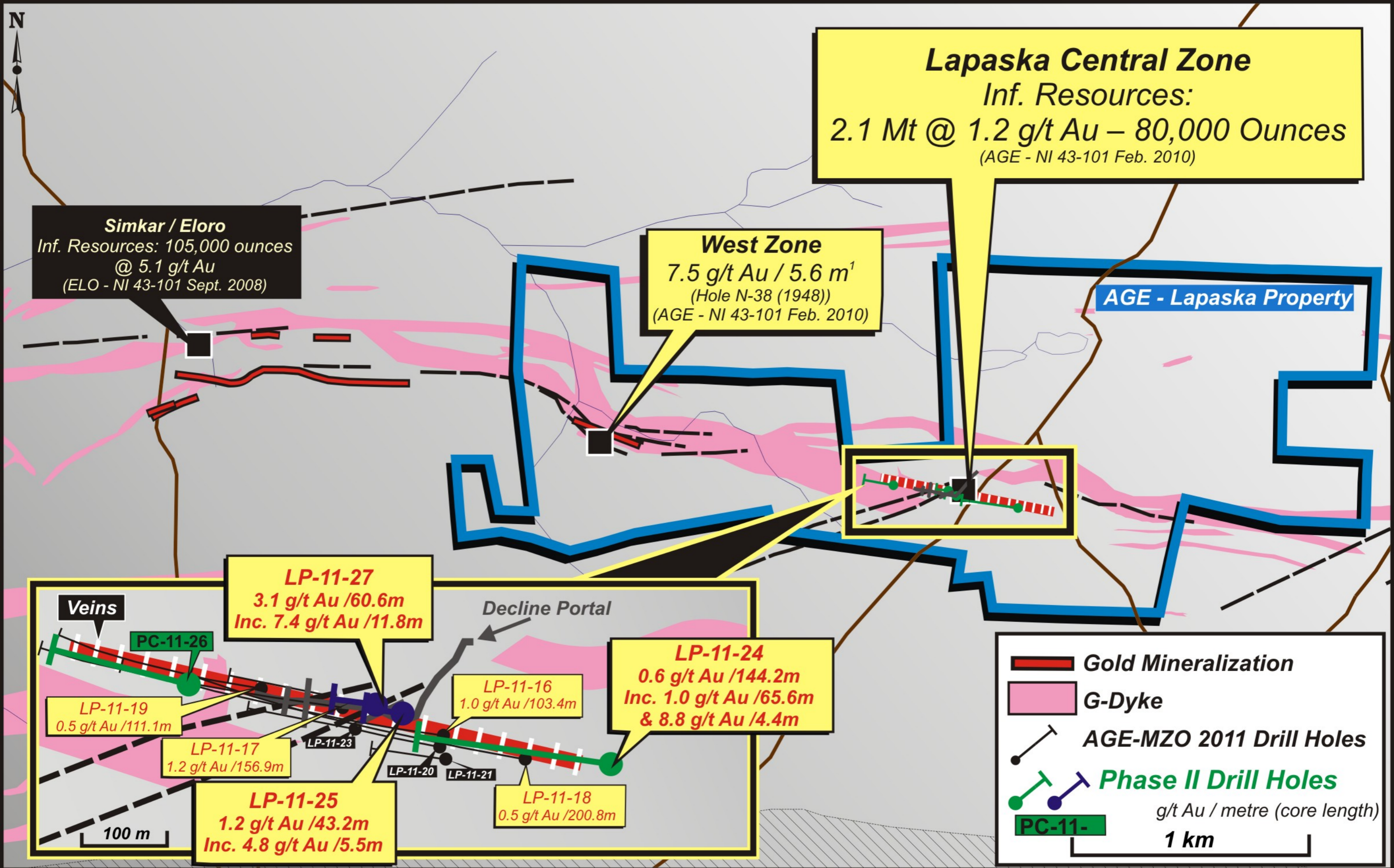
Figure 1: Surface Map - Phase II Preliminary Results - Lapaska Property
